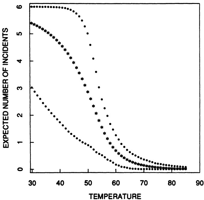
Figure 13. Binomial-Logit Model (Temperature and Pressure). Pressure: 200 psi.
