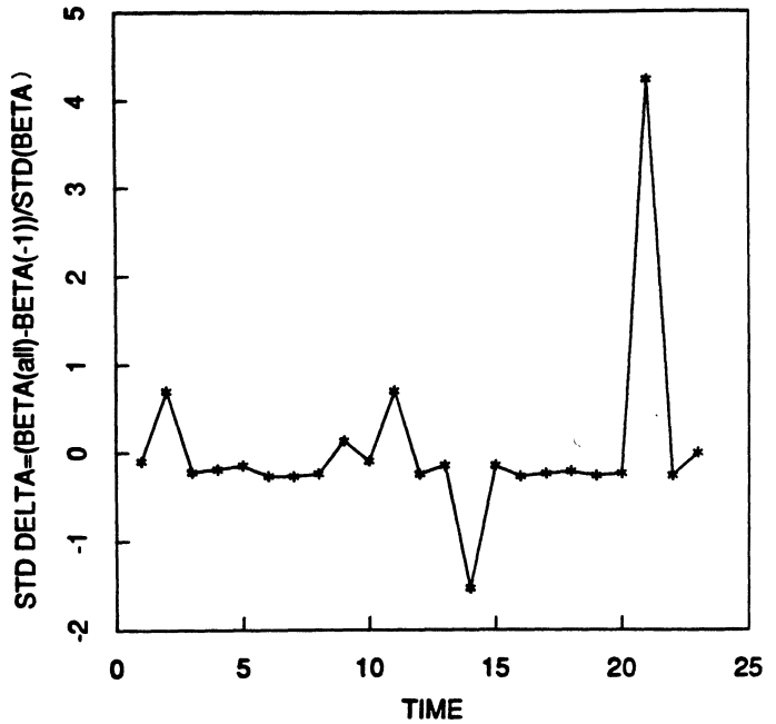
Figure 6. Delta Beta Plot and Binomial-Logit Model: N = 6 .
