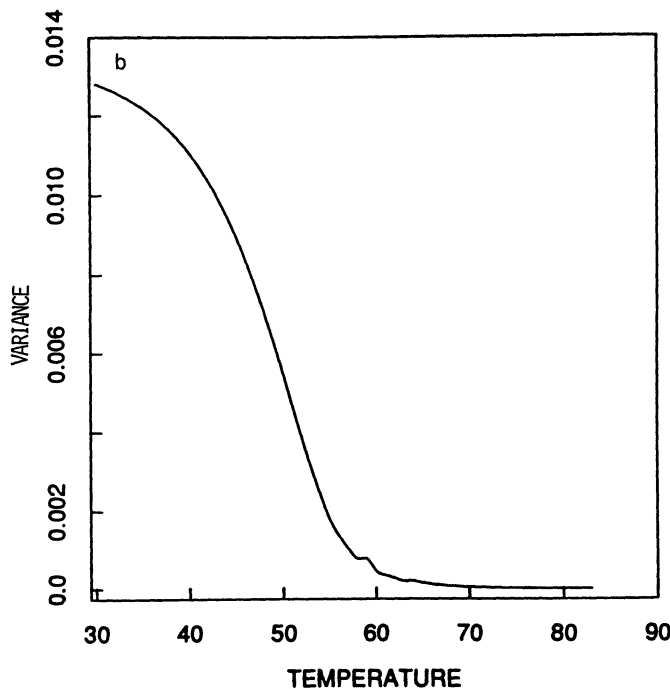
Figure 18. (a) Means and (b) Variances of Fitted Beta Distributions Versus Temperature.
